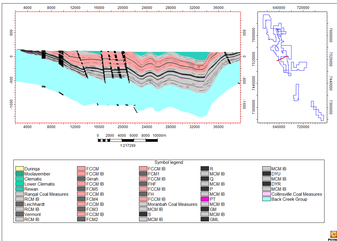
Figure 7 : Stratigraphy underlying ATP 1031
