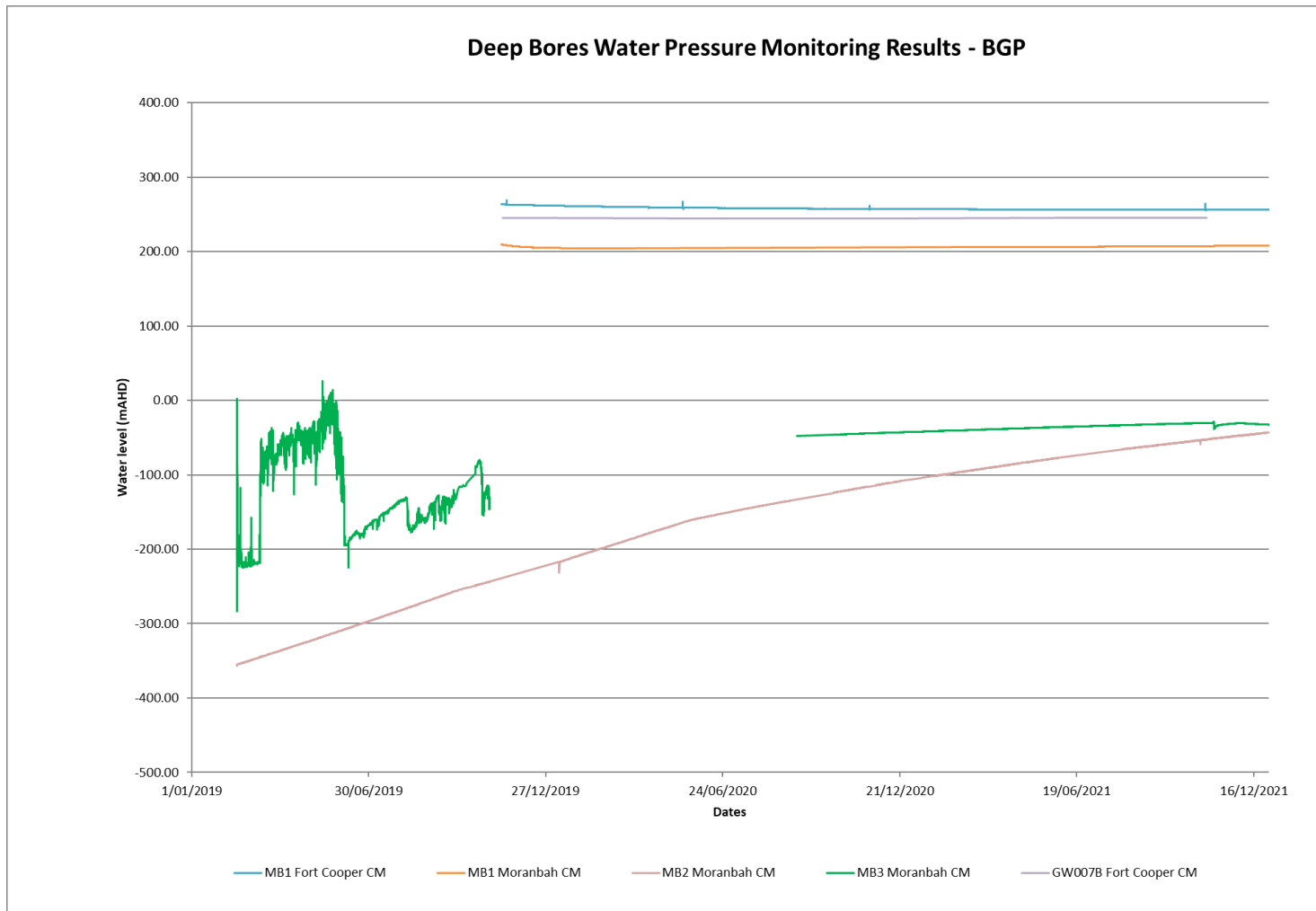
Figure 13: Deep Bores Water Level Monitoring Results - BGP
