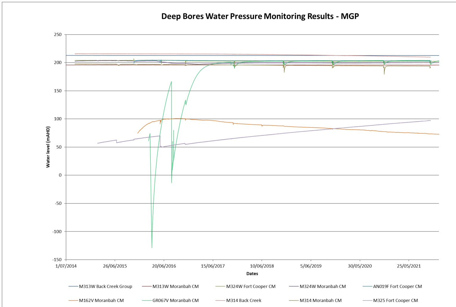
Figure 12: Deep Bores Water Level Monitoring Results - MGP
