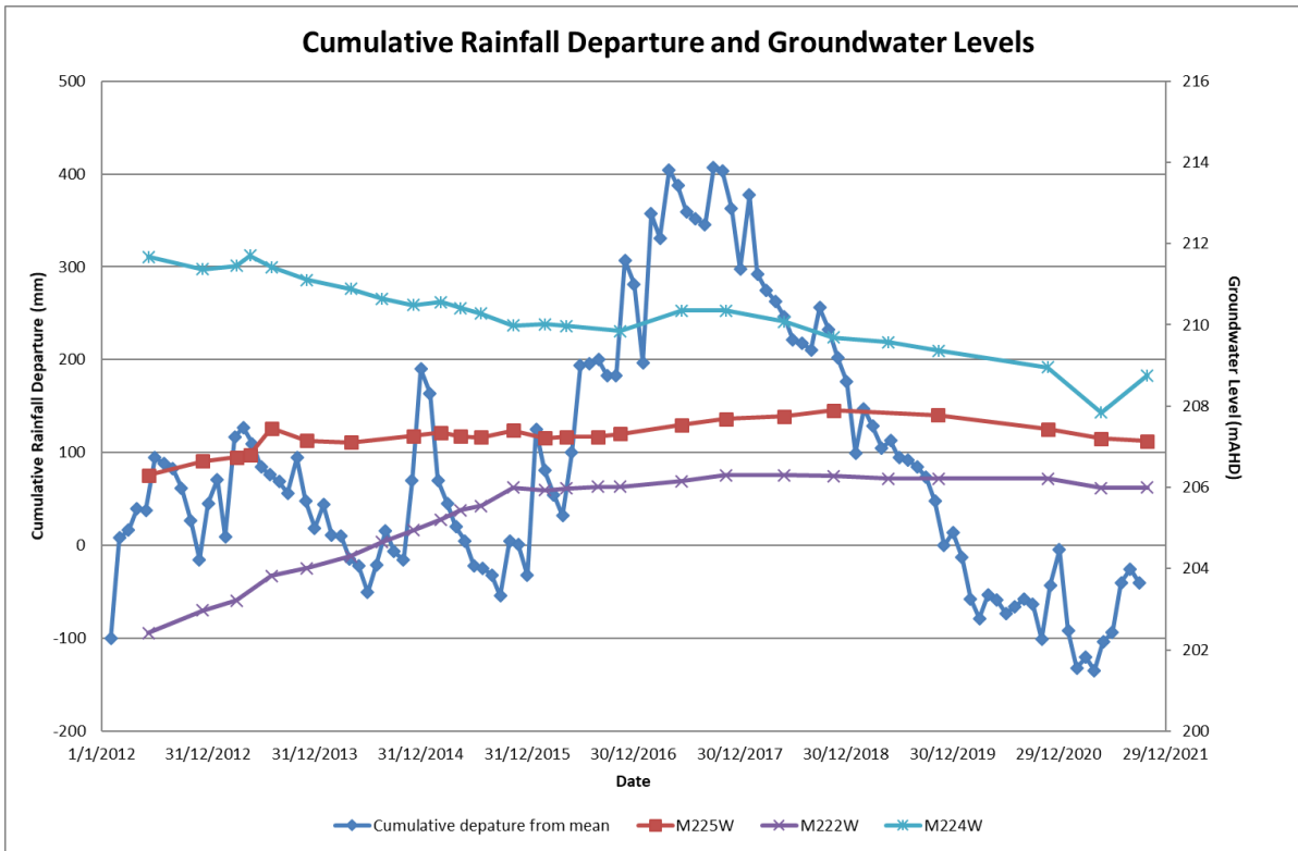
Figure 7: Cumulative Rainfall Departure and Groundwater Levels
