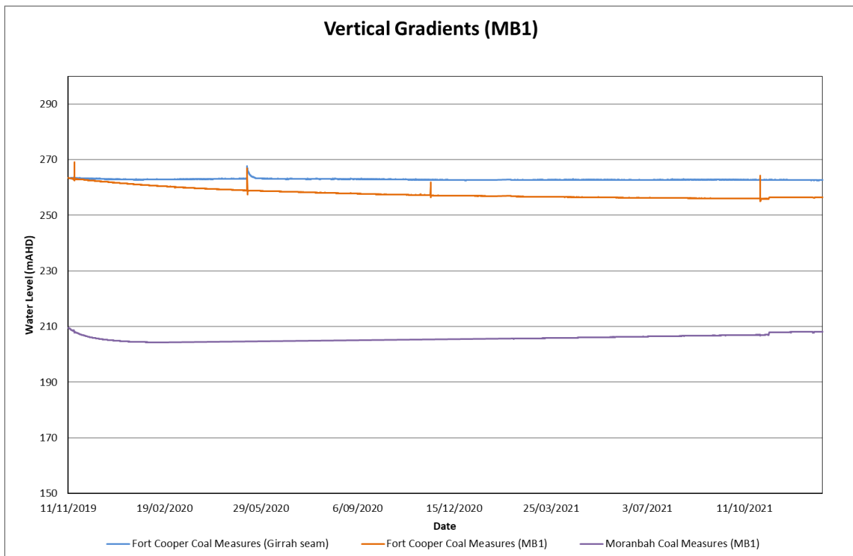
Figure 14: Site 3 - Review of Vertical Gradients (MB1)
