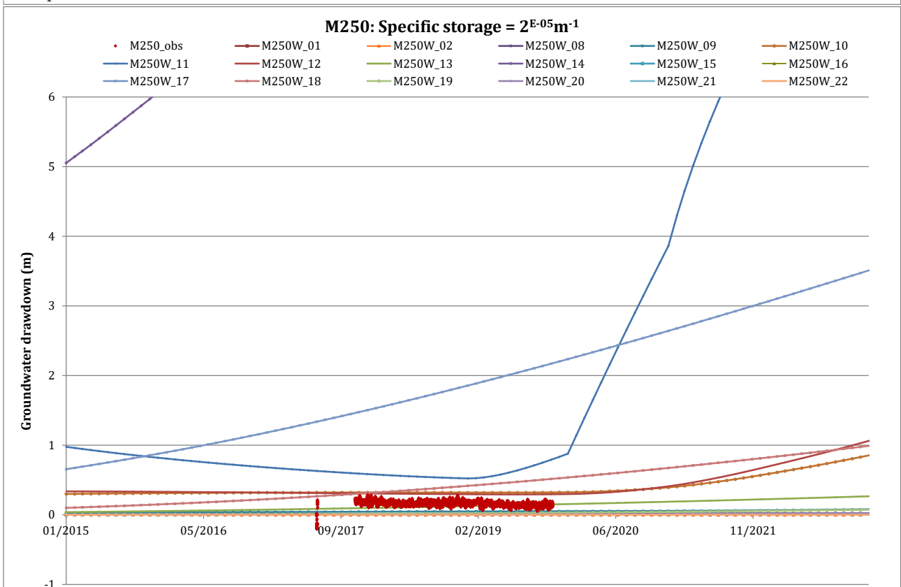
Figure 5.6 M250 drawdown comparison
