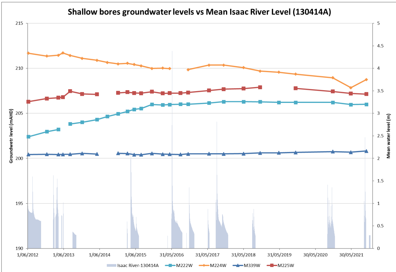
Figure 8: Shallow Groundwater levels vs mean Isaac River levels
