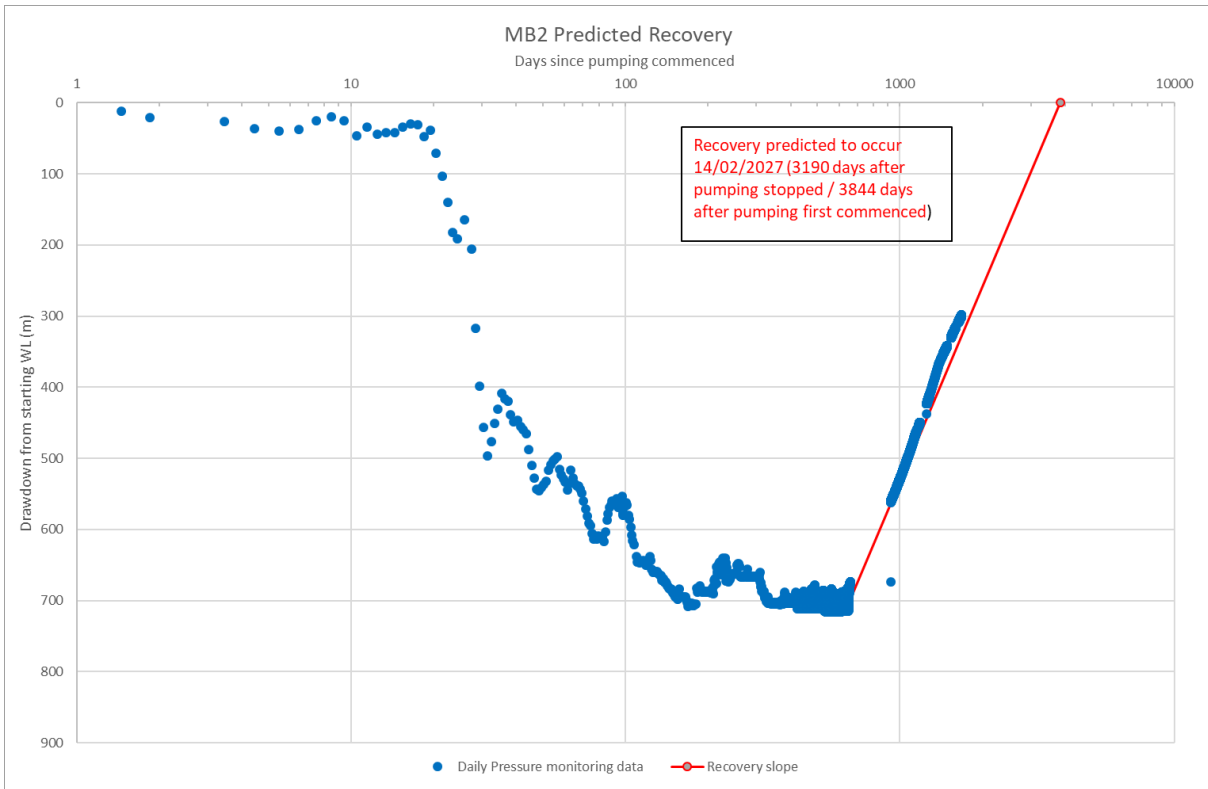
Figure 10: MB2 recovery data
